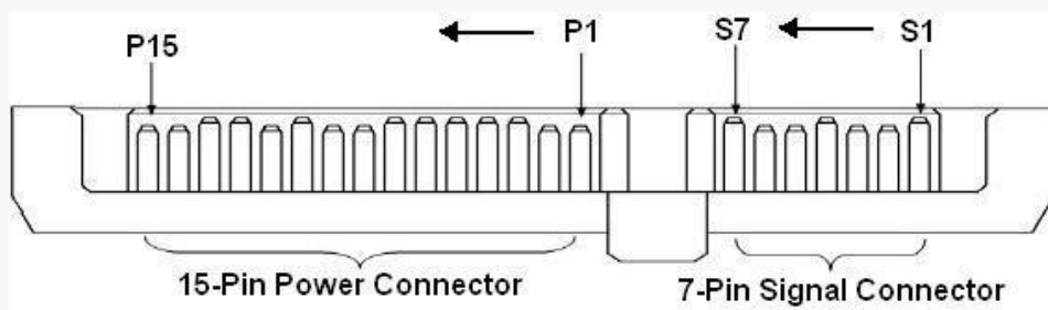
Figure 2: 7+15 Serial ATA port Interface Description
