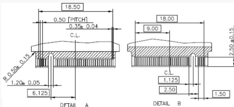
Figure 2: M.2 Interface Description
